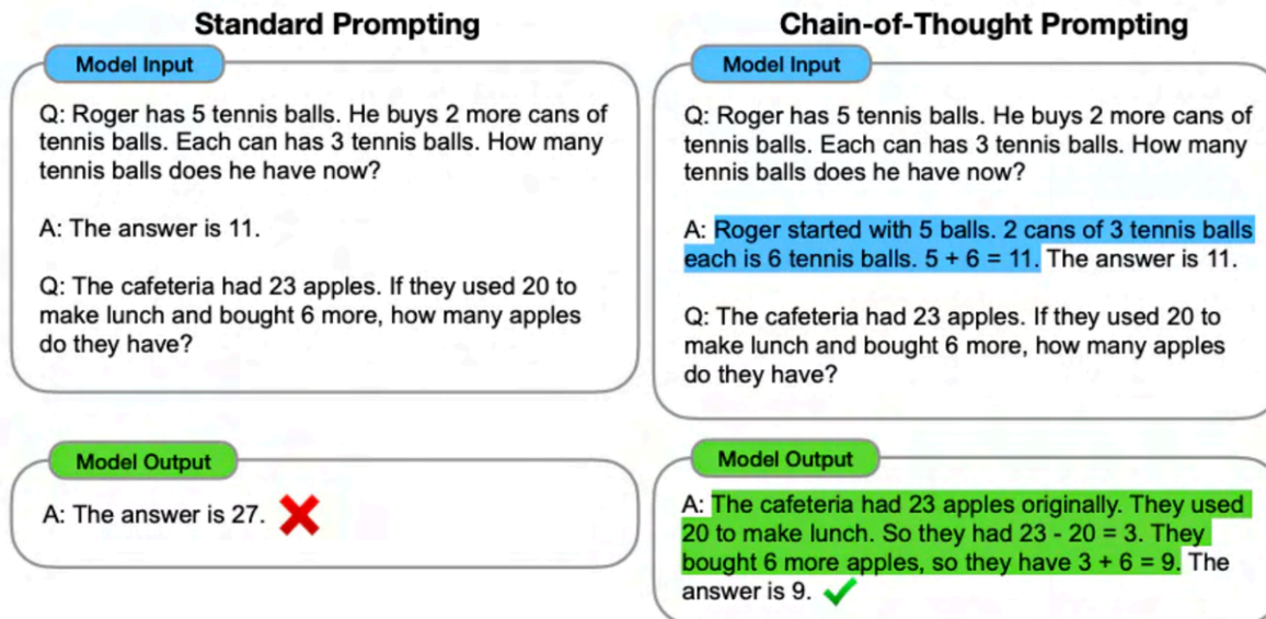
Figure 29. Standard Prompting and Chain-of-Thought Prompting (Wei and Zhou 2022).
