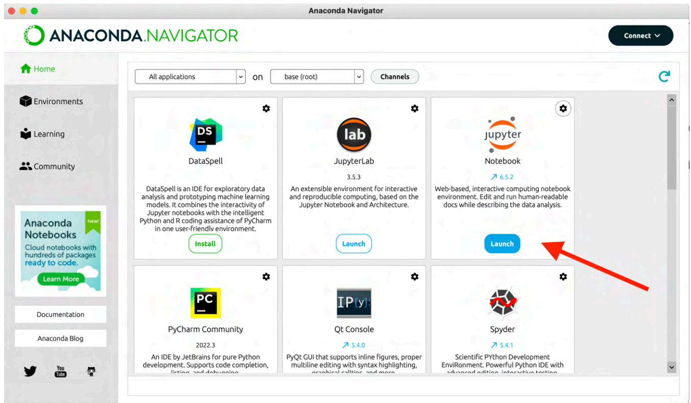
Figure 35. Anaconda Navigator.
