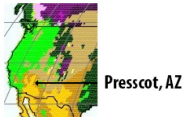
Figure 43: Prescott, AZ on Koppen Climate Map and Projected Climate Map
