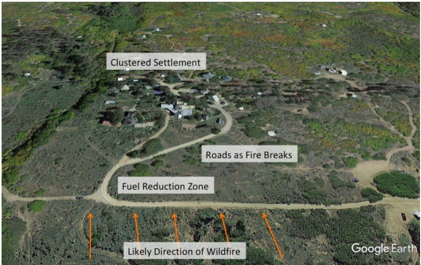
Figure 61: Site Plan Diagram
