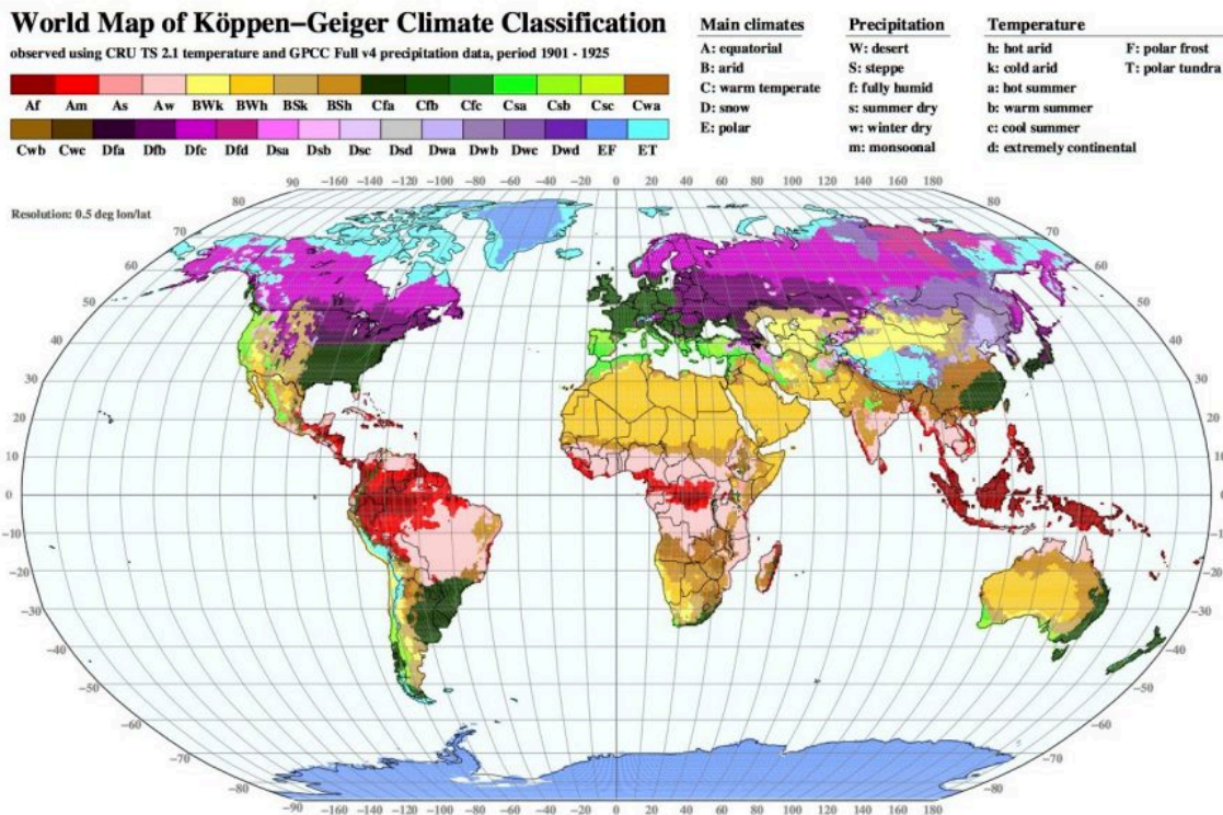
Figure 1: World Map of Köppen-Geiger Climate Classification observed using CRU TS 2.1 temperature and GPCP Full v4 precipitation data, period 1901 - 1925 on a regular 0.5 degree latitude/longitude grid.
