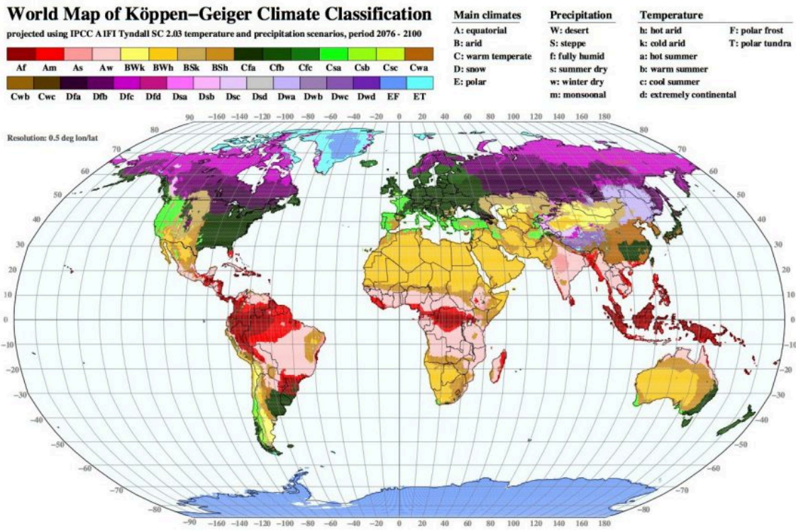
Figure 2: World Map of Köppen–Geiger climate classification projected with Tyndall temperature and precipitation data for the period 2076–2100, A1FI emission scenario, on a regular 0.5 degree latitude/longitude grid.
