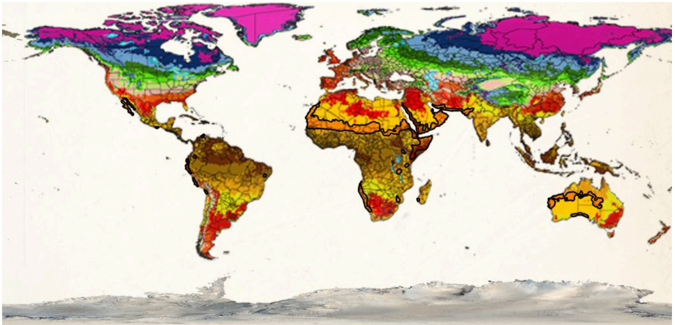
Figure 24: Koppen Geiger map with plant hardiness zones overlaid. Orange areas surrounded by black lines are areas of overlap between the Koppen Geiger classification and the plant hardiness zone.
