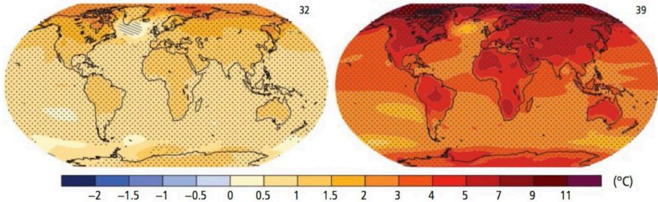
Figure 32: Change in Average Surface Temperature (1986–2005 to 2081–2100)
