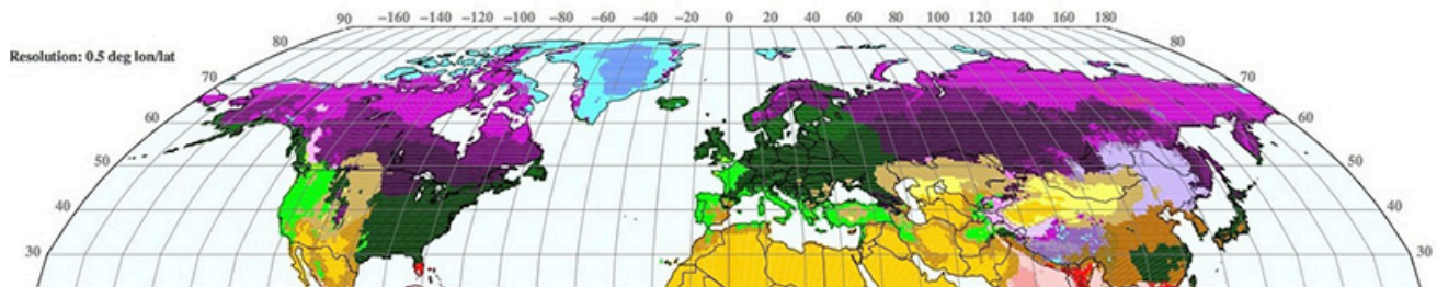
Projected Northern Hemisphere 2076-2100
